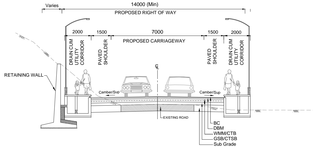
TCS 10 TYPICAL CROSS SECTION FOR 2 LANE IN HALF CUT WITH RETAINING WALL - LHS
