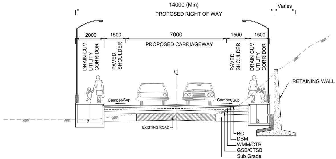
TCS 5A TYPICAL CROSS SECTION FOR 2 LANE IN HALF CUT IN EXISTING WITH RETAINING WALL - RHS
