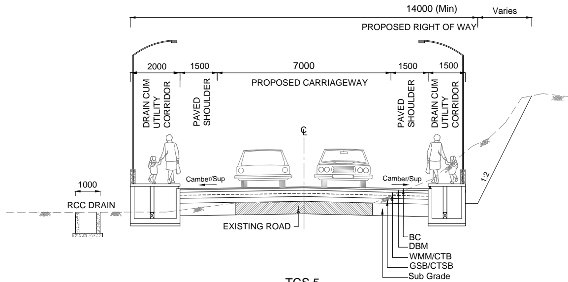
TCS 5 TYPICAL CROSS SECTION FOR 2 LANE WITH HALF CUT IN EXISTING - RHS (BUILT UP SECTION)
