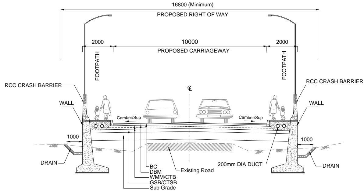
TCS 3A TYPICAL CROSS SECTION FOR 2 LANE IN EXISTING WITH RETAINING WALL ON MERGING SECTION
