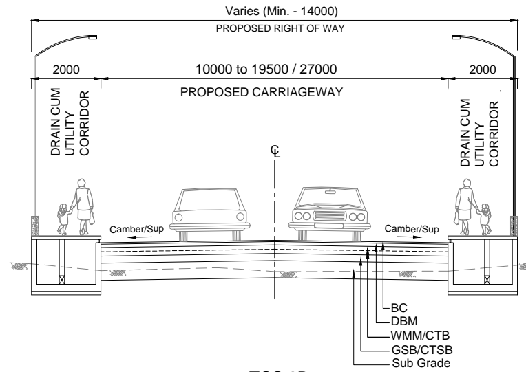
TCS 2B TYPICAL CROSS SECTION FOR 2 ~ 4 LANE MERGING SECTION IN GREEN FIELD
