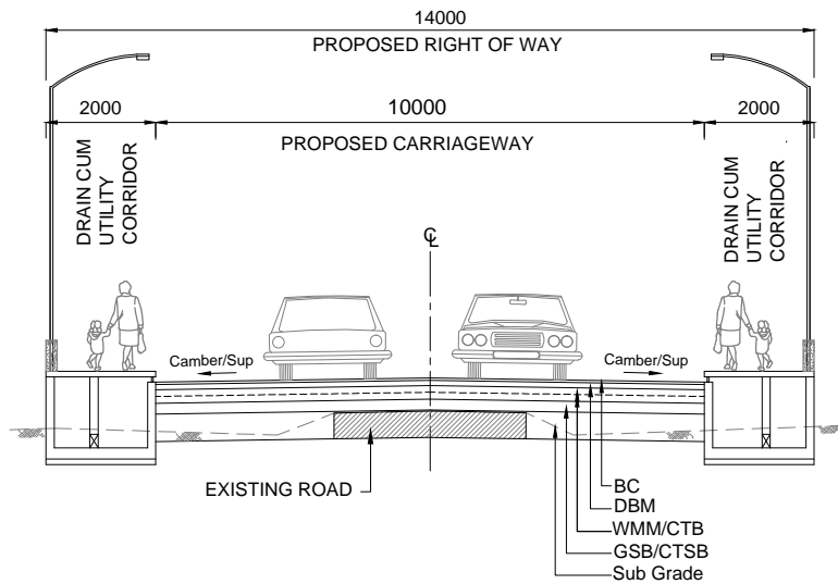
TCS 1 TYPICAL CROSS SECTION FOR 2 LANE IN EXISTING SECTION
