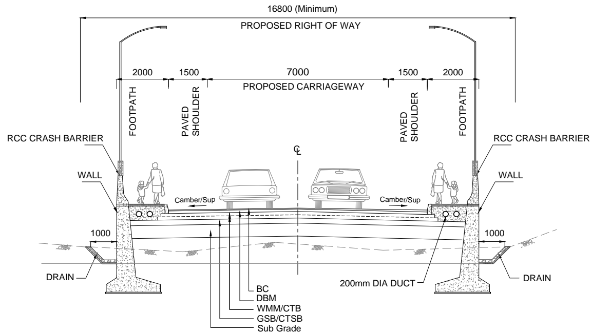
TCS 3 TYPICAL CROSS SECTION FOR 2 LANE IN GREEN FIELD (HIGH EMBANKMENT)
