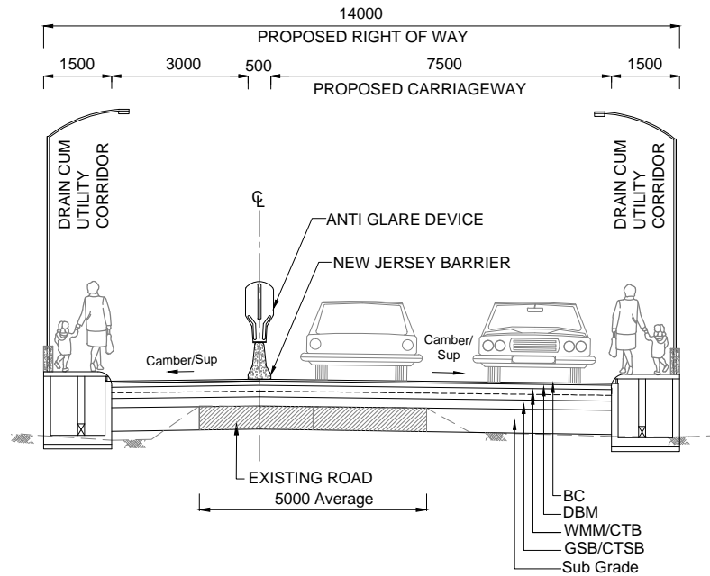
TCS 15C TYPICAL CROSS SECTION FOR 2 LANE WITH CYCLE TRACK ON BUILT UP SECTION
