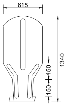
TYPICAL DETAILS OF ANTI GLARE DEVICE
