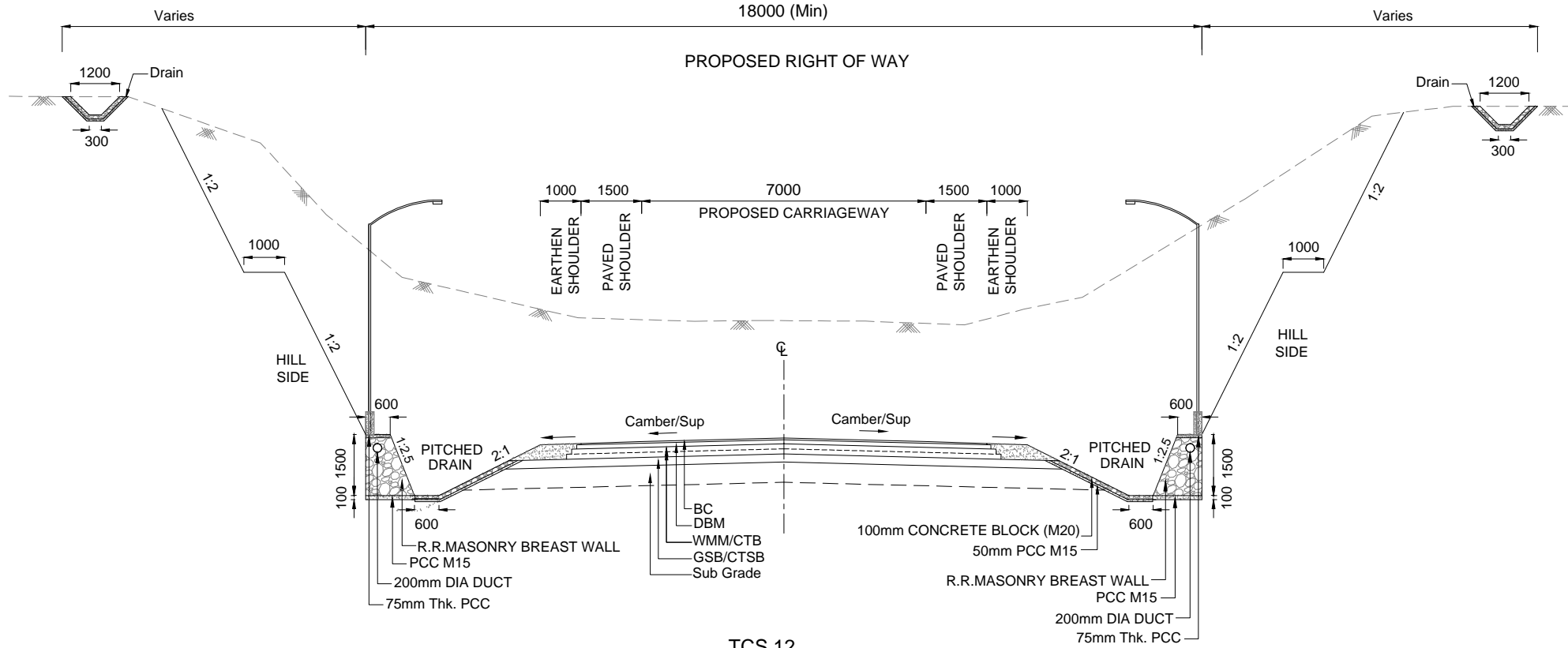
TCS 12 TYPICAL CROSS SECTION - 2 LANE GREEN FIELD BOX CUT - HILL
