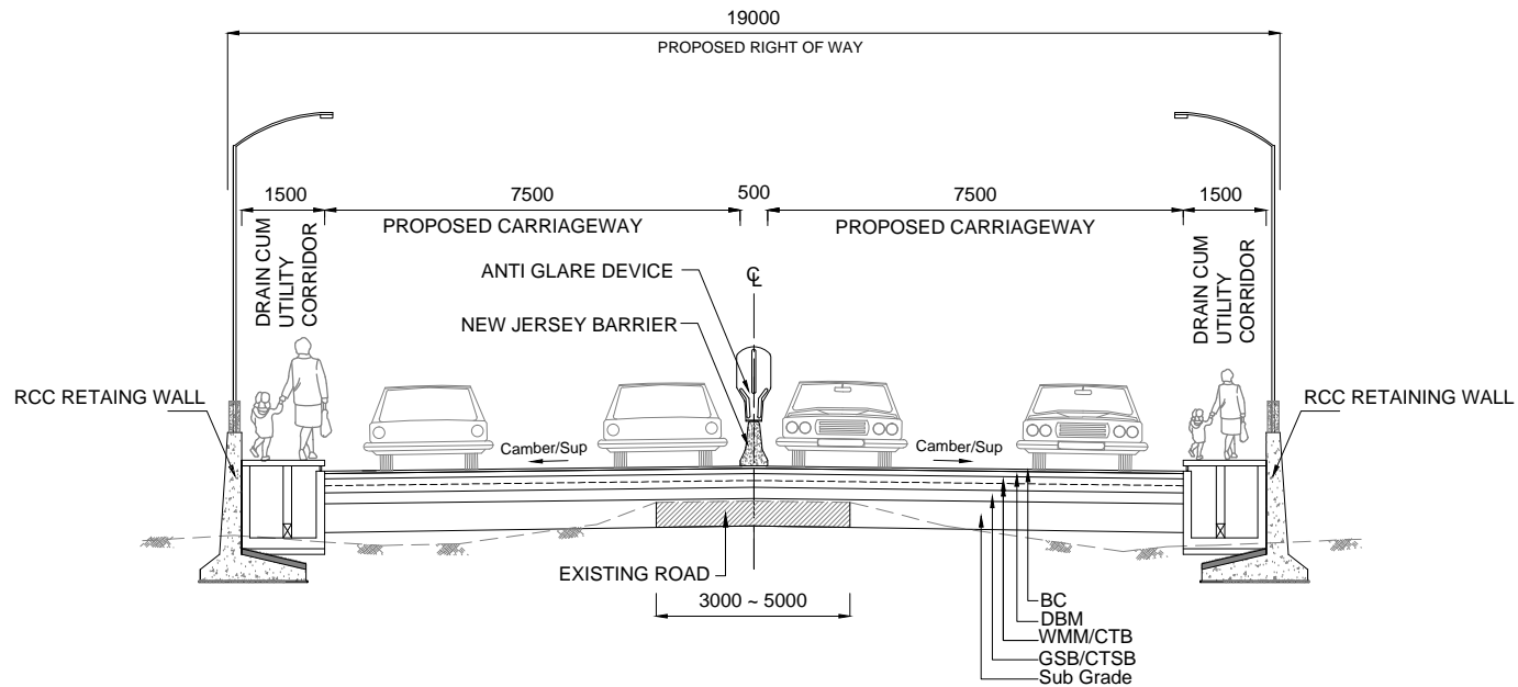
TCS 7 TYPICAL CROSS SECTION FOR 4 LANE DIVIDED CARRIAGEWAY WITHOUT SERVICE ROAD ON HIGH EMBANKMENT SECTION
