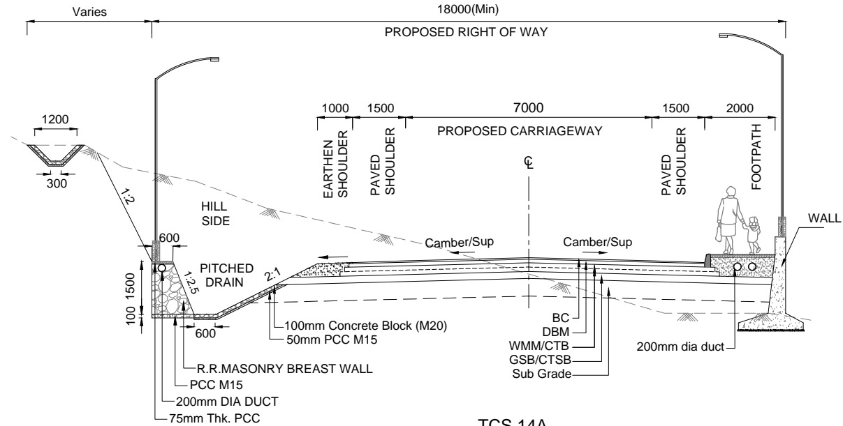
TCS 14A TYPICAL CROSS SECTION - 2 LANE ON EXISTING WITH HALF CUT - LHS & HIGH EMBANKMENT ON RHS
