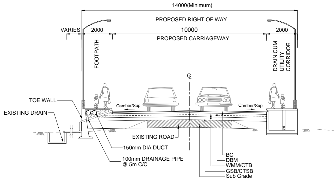
TCS 3C TYPICAL CROSS SECTION FOR 2 LANE IN EXISTING DRAIN (LHS) WITH TOE WALL
