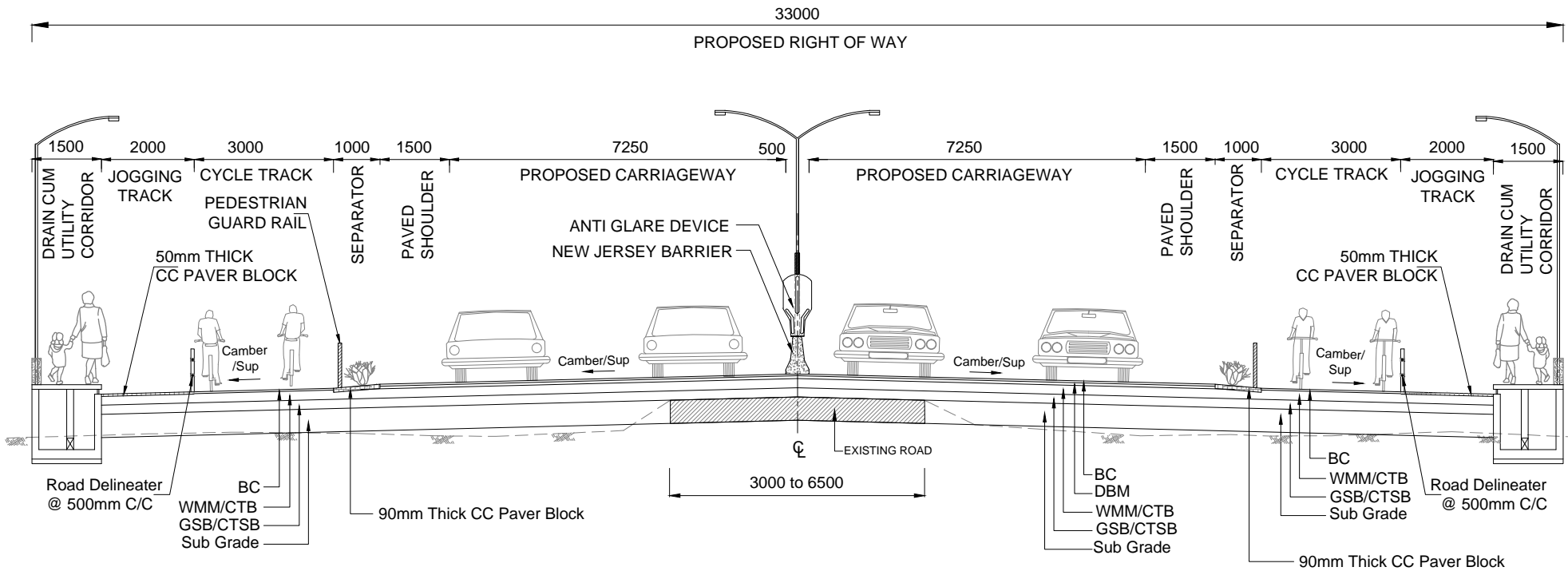
TCS 9 TYPICAL CROSS SECTION FOR 4 LANE DIVIDED CARRIAGEWAY WITH BOTH SIDE CYCLE TRACK
