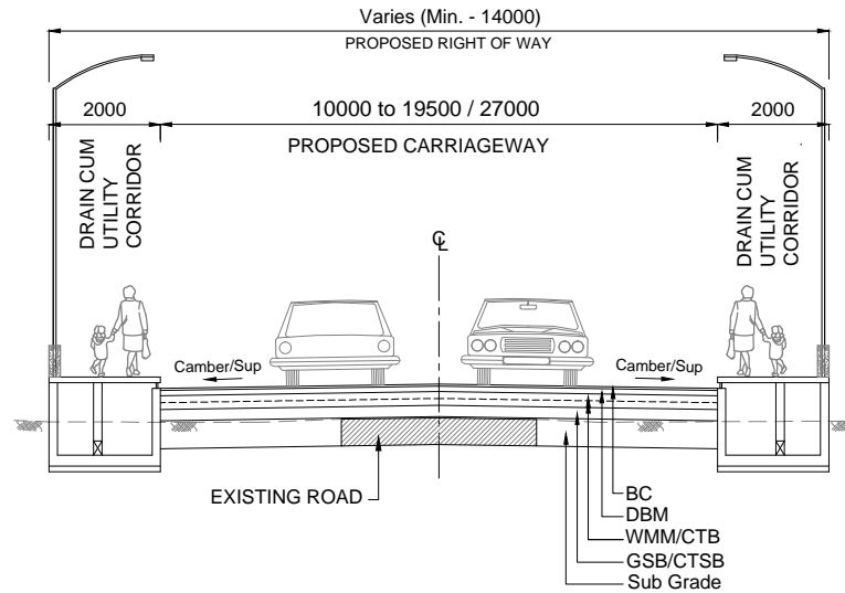
TCS 1A TYPICAL CROSS SECTION FOR 2 ~ 4 LANE MERGING SECTION IN EXISTING SECTION
