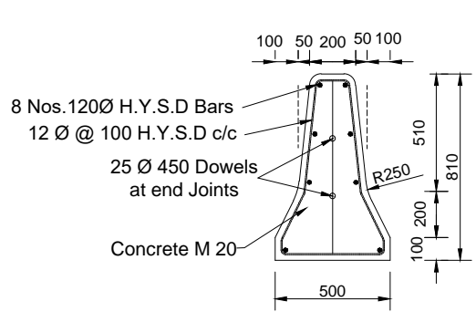
NEW JERSEY BARRIER
