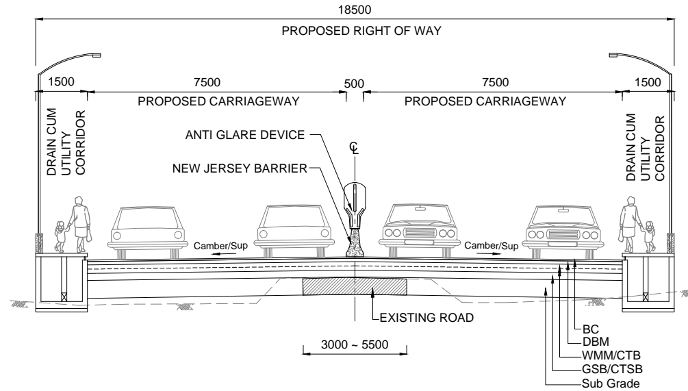
TCS 8 TYPICAL CROSS SECTION FOR 4 LANE DIVIDED CARRIAGEWAY WITHOUT SERVICE ROAD (EXITING ROAD SECTION)
