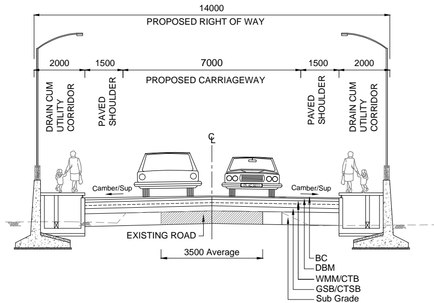
TCS 15B TYPICAL CROSS SECTION ON EXISTING WITH RETAINING WALL BOTH SIDE
