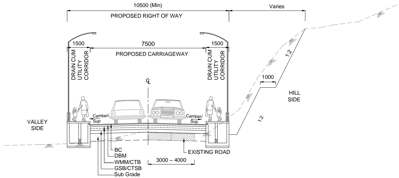
TCS 13B TYPICAL CROSS SECTION - 2 LANE IN RESTRICTED AREA WITH HALF CUT - RHS
