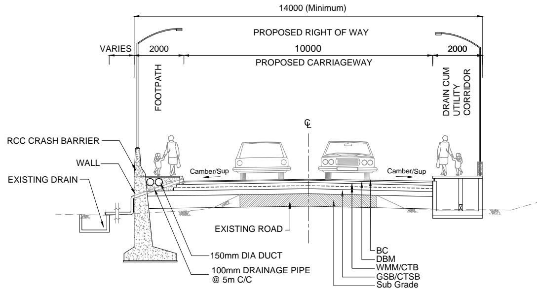
TCS 3B TYPICAL CROSS SECTION FOR 2 LANE IN EXISTING DRAIN (LHS) SECTION
