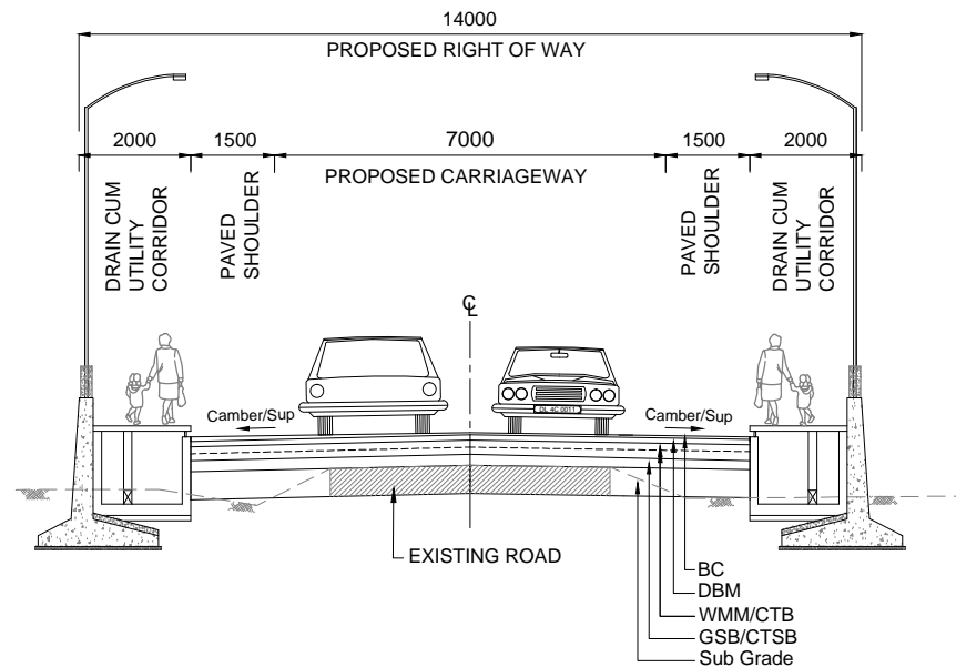
TCS 15F TYPICAL CROSS SECTION FOR 2 LANE ON EXISTING SECTION WITH RETAINING WALL - BOTH
