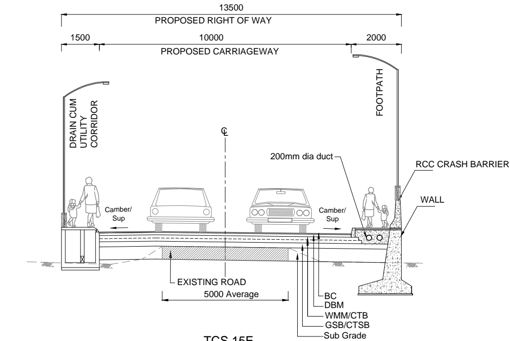
TCS 15E TYPICAL CROSS SECTION FOR 2 LANE ON EXISTING SECTION ( WITH EXISTING NALA) WITH RETAINING WALL - RHS
