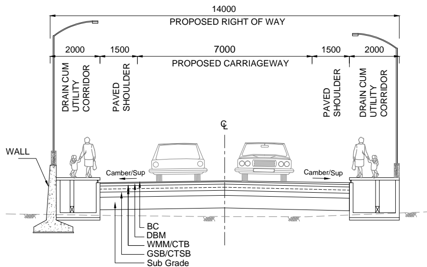
TCS - 2A TYPICAL CROSS SECTION FOR 2 LANE IN GREEN FIELD SECTION WITH RETAINING WALL - LHS
