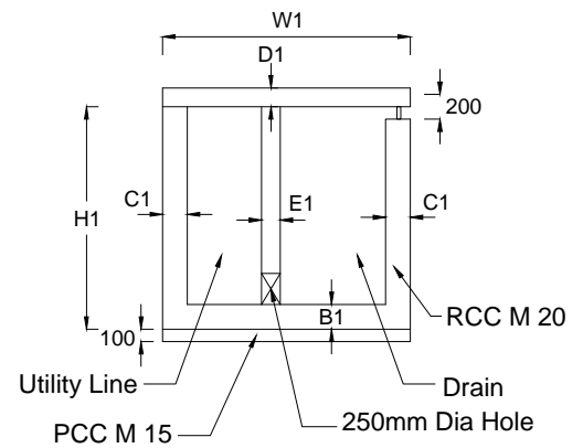
DRAIN CUM UTILITY CORRIDOR - C
