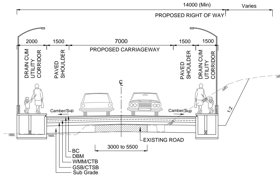
TCS 4 TYPICAL CROSS SECTION FOR 2 LANE WITH HALF CUT IN EXISTING SECTION (RHS)
