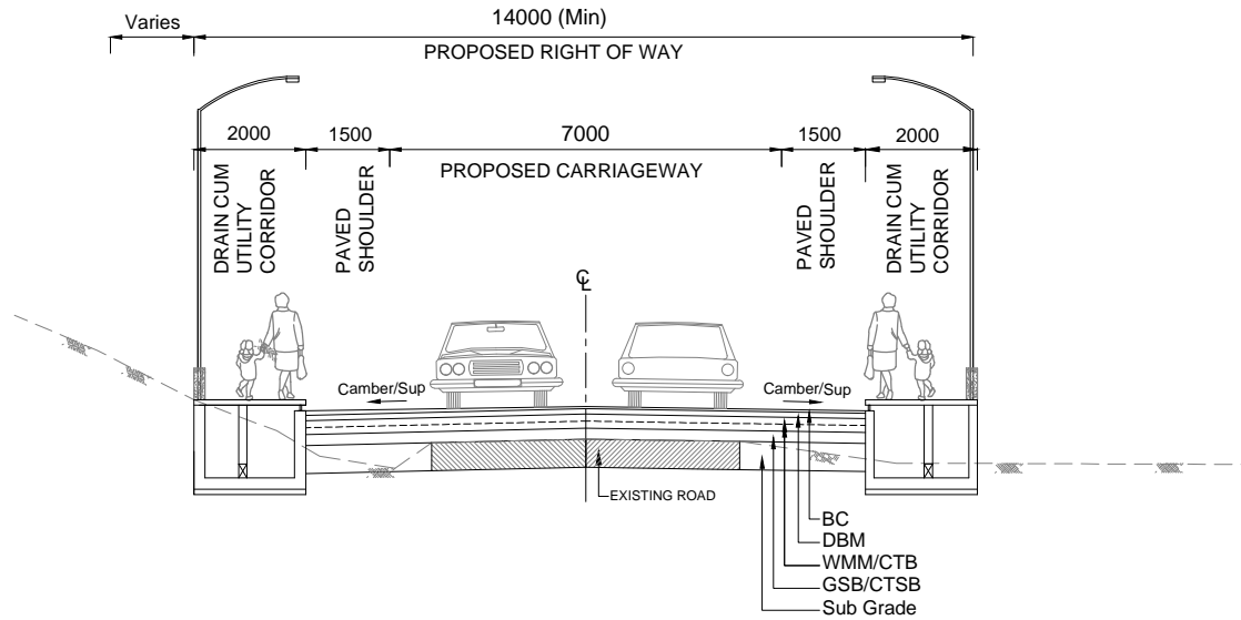
TCS 10A TYPICAL CROSS SECTION FOR 2 LANE IN HALF CUT WITHOUT RETAINING WALL - LHS
