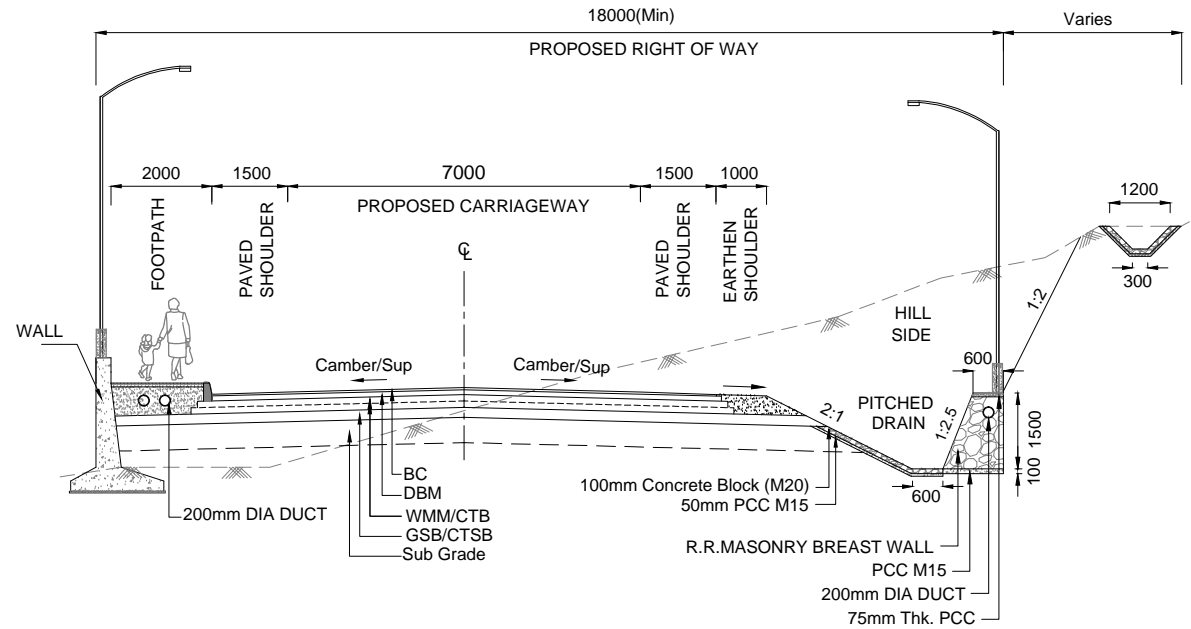
TCS 14 TYPICAL CROSS SECTION - 2 LANE WITH HALF CUT - RHS & HIGH EMBANKMENT ON LHS
