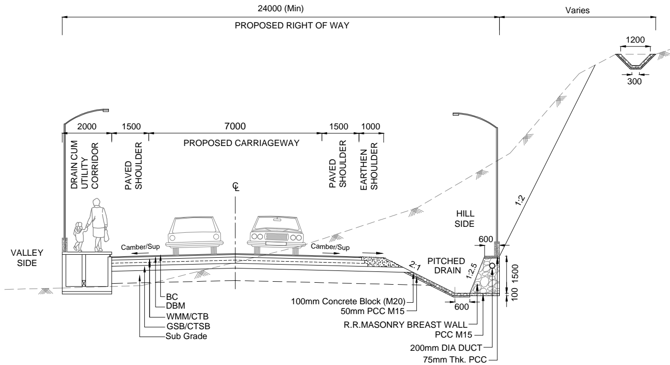
TCS 13 TYPICAL CROSS SECTION - 2 LANE GREEN FIELD WITH HALF CUT - RHS
