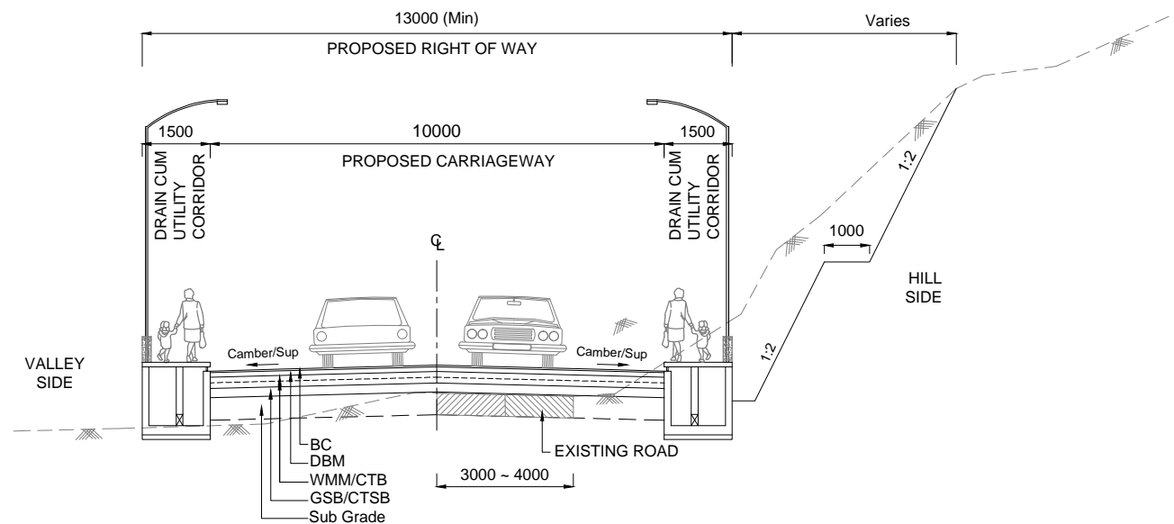
TCS 13A TYPICAL CROSS SECTION - 2 LANE IN BUILT UP SECTION WITH HALF CUT - RHS
