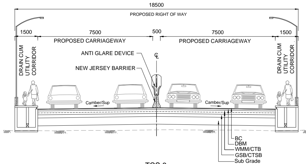
TCS 6 TYPICAL CROSS SECTION FOR 4 LANE DIVIDED CARRIAGEWAY WITHOUT SERVICE ROAD (GREEN FIELD SECTION)
