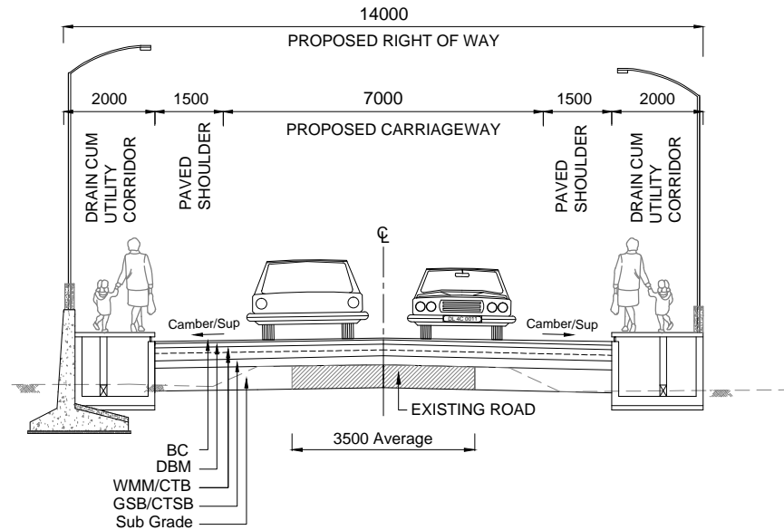
TCS 15A TYPICAL CROSS SECTION FOR 2 LANE ON EXISTING WITH RETAINING WALL - LHS
