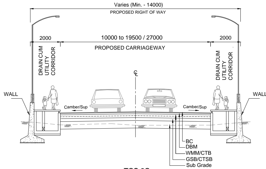
TCS 2C TYPICAL CROSS SECTION FOR 2 ~ 4 LANE MERGING SECTION IN GREEN FIELD WITH BOTHSIDE RETAINING WALL
