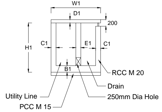
DRAIN CUM UTILITY CORRIDOR - B
