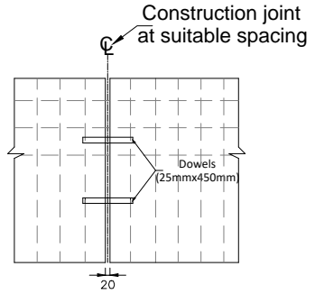
JOINT DETAIL OF NEW JERSEY BARRIER
