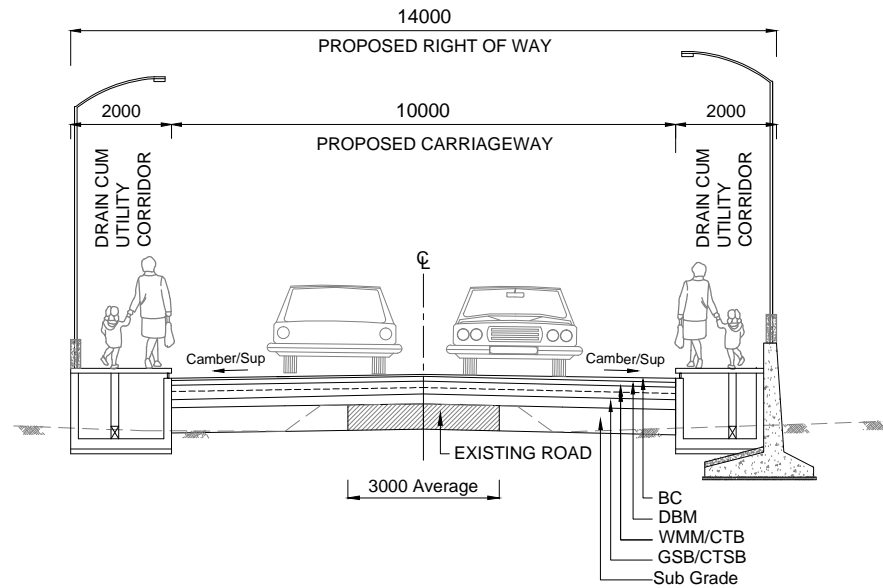
TCS 15D TYPICAL CROSS SECTION FOR 2 LANE ON EXISTING SECTION WITH RETAINING WALL - RHS
