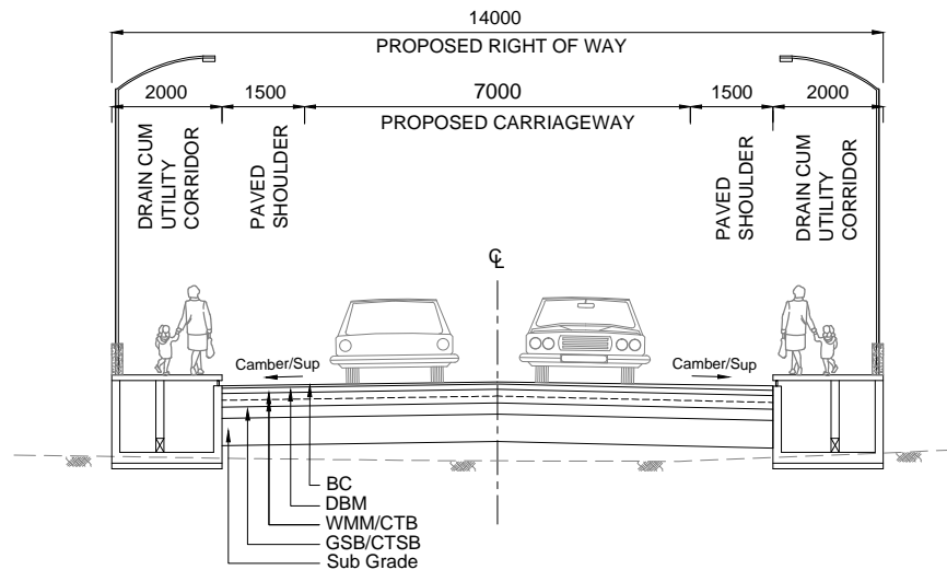
TCS - 2 TYPICAL CROSS SECTION FOR 2 LANE IN GREEN FIELD SECTION
