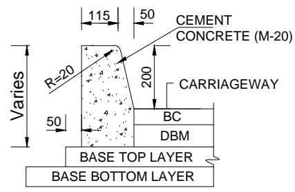
SECTION OF BARRIER TYPE KERB
