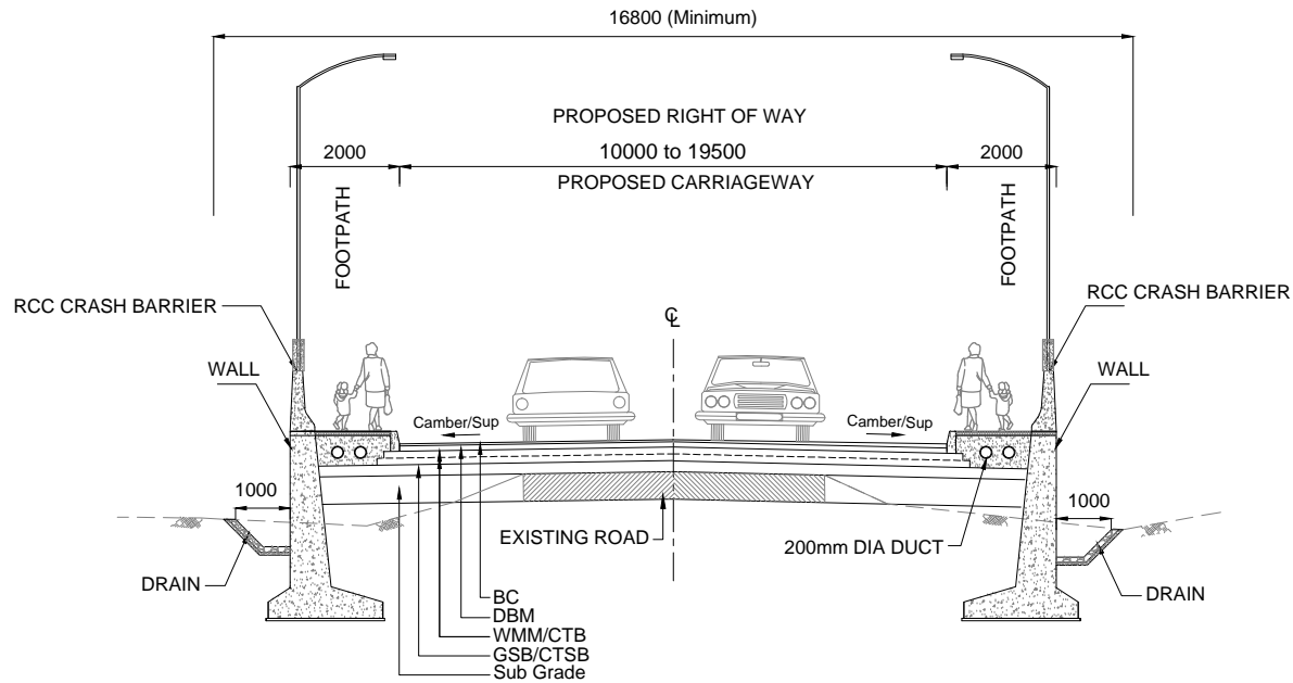
TCS 3D TYPICAL CROSS SECTION FOR 2 LANE IN EXISTING ON HIGH EMBANKMENT ON MERGING SECTION
