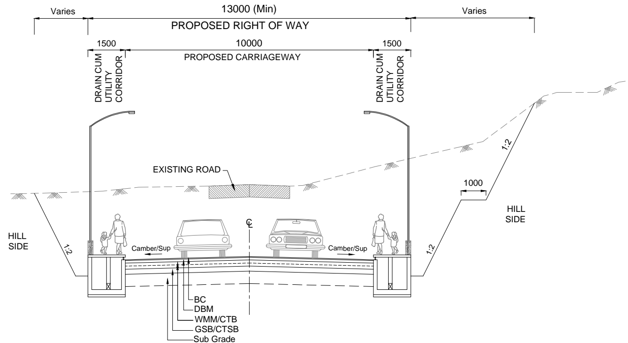
TCS 12A TYPICAL CROSS SECTION - 2 LANE IN EXISTING SECTION IN BOX CUT - HILL
